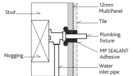
Figure 1 — Detail of sealing wall penetration NOTE — Apply a continuous bead of MP SEALANT Adhesive to all corner and vertical flashings.
