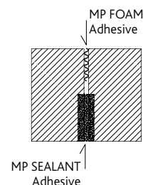
Figure 1 — Detail of sealing wall penetration NOTE — Apply a continuous bead of MP SEALANT Adhesive to all corner and vertical flashings.
