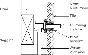
Figure 1 — Detail of sealing wall penetration NOTE — Apply a continuous bead of FIX30 sealant to all corner and vertical flashings
